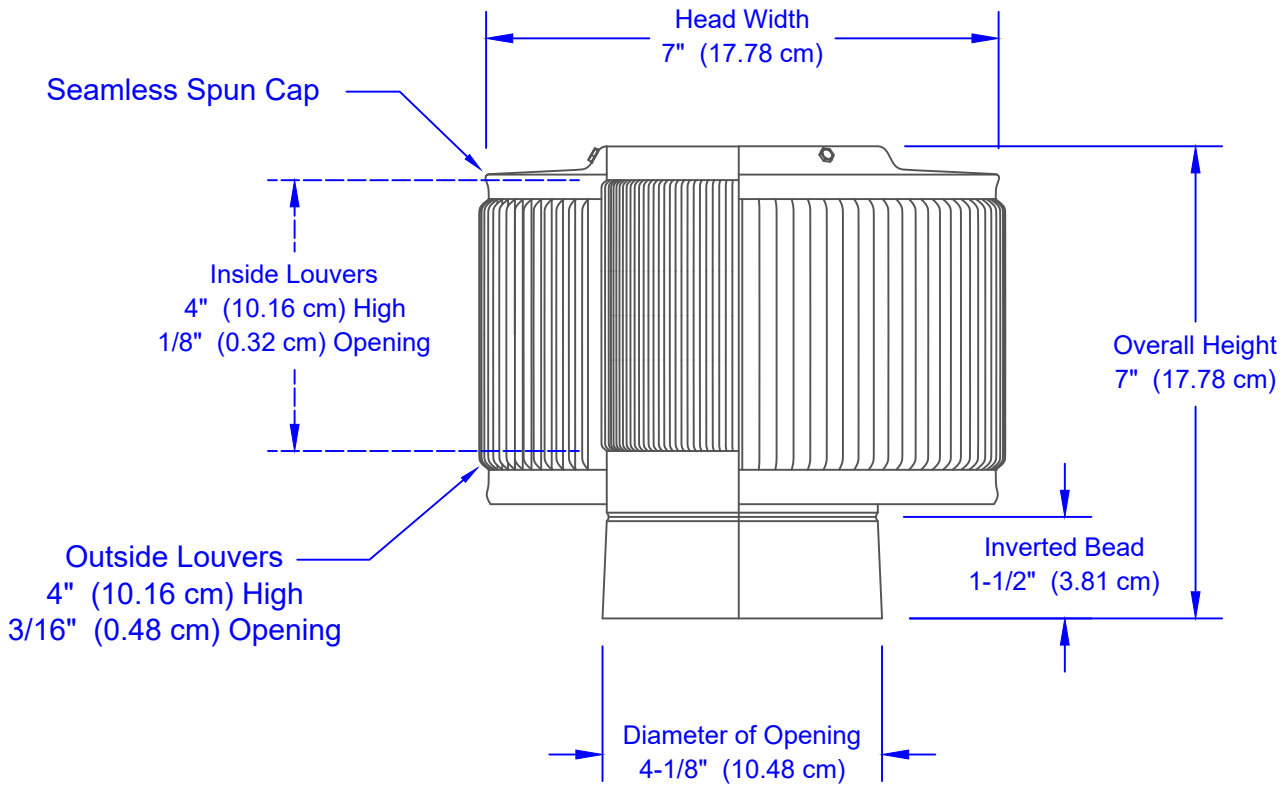
Cut-away View
