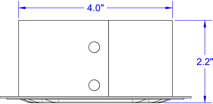
Side View
