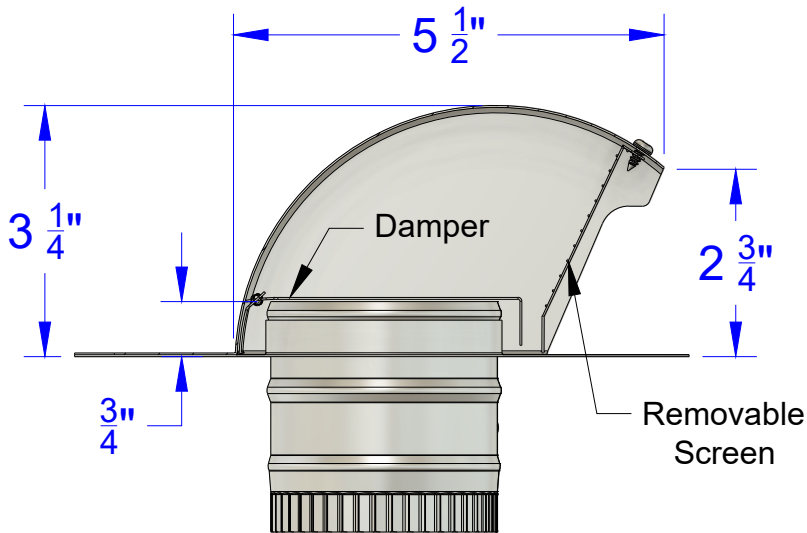
Side Section View
