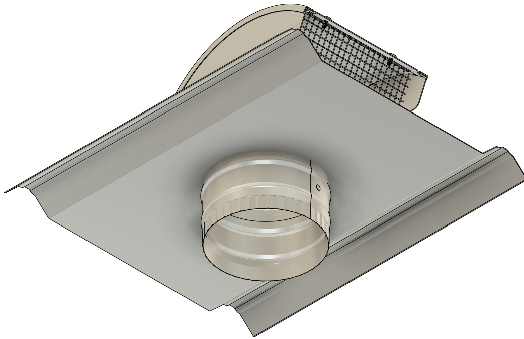
Angle Bottom View showing Tail Pipe for Duct
