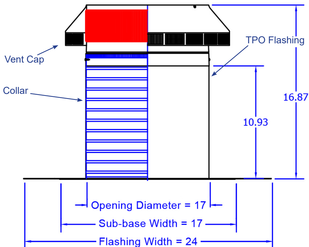
View of flashing going over sub-base
