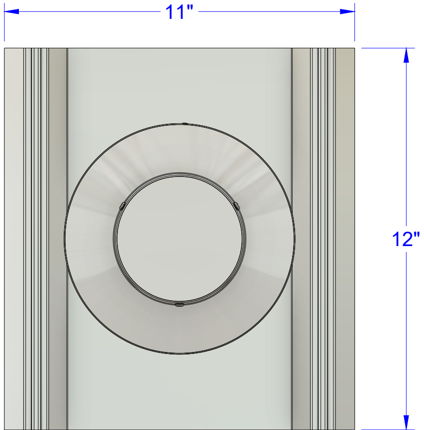
Top View
