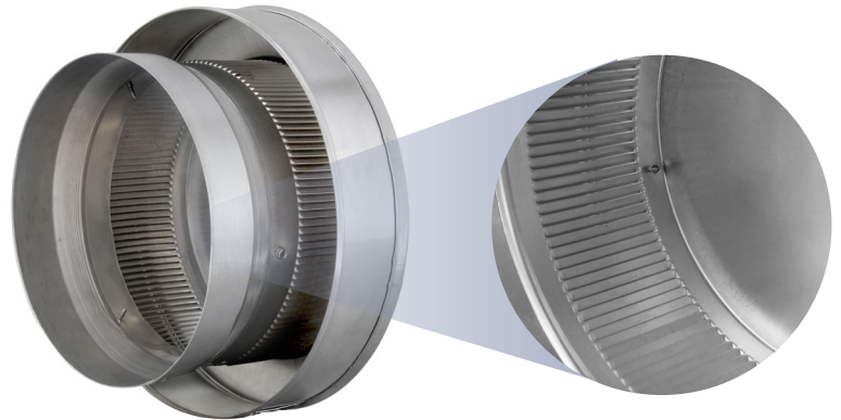
Close up view of 1/8" louvers
