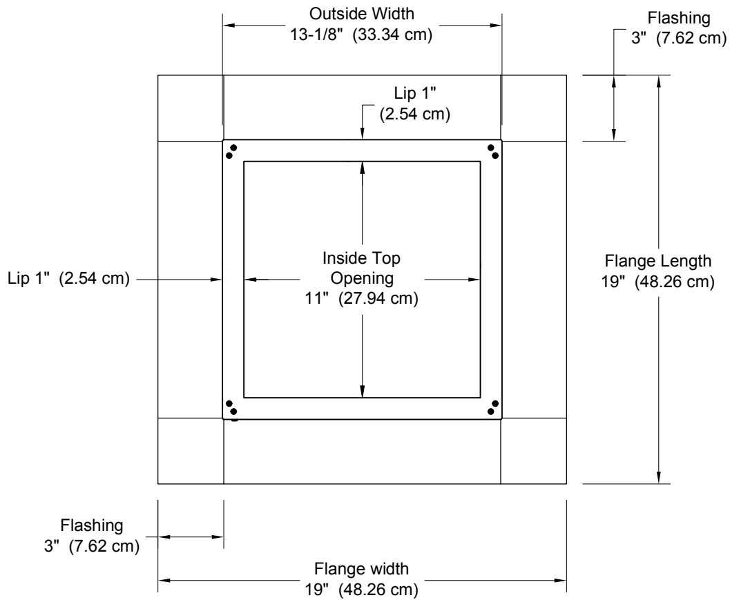
Top View
