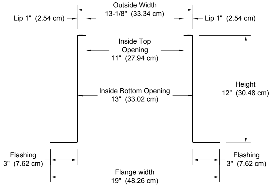
Side View
