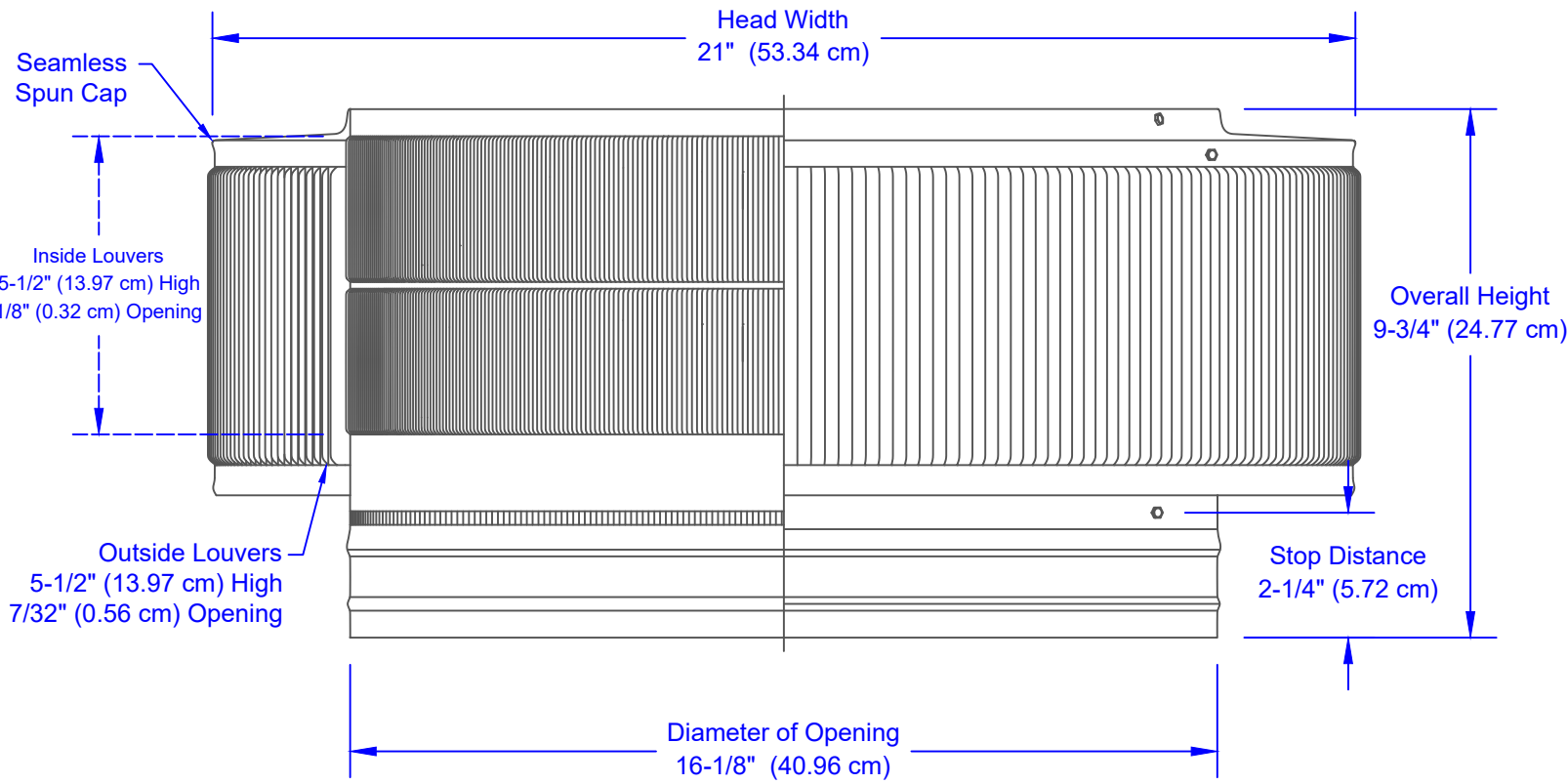
Cut-away View
