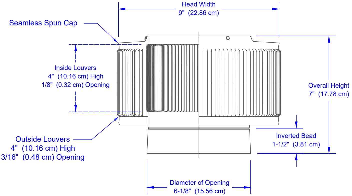
Cut-away View
