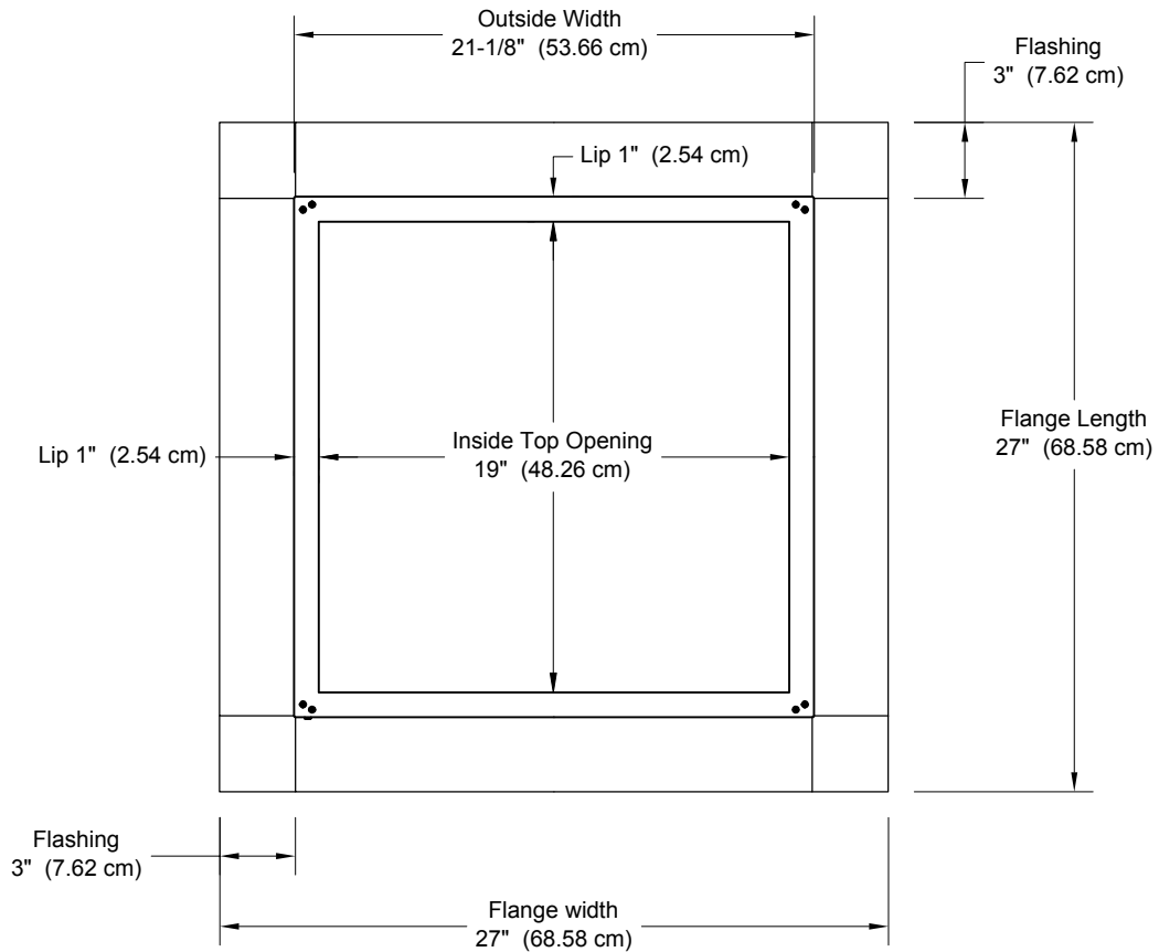
Top View
