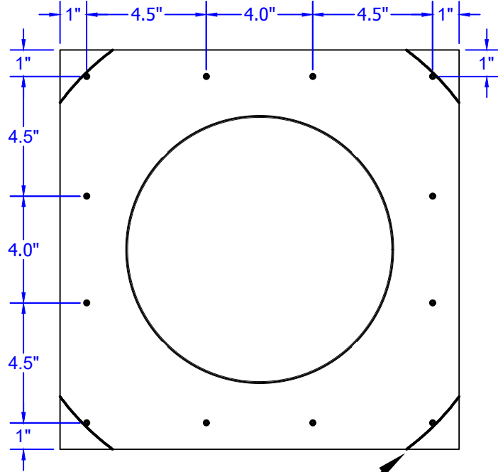
Rounded Corner option
